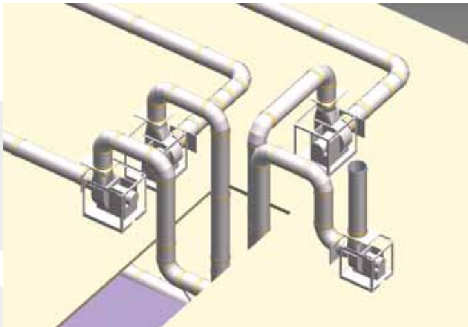
Ventilation planning drawings.
